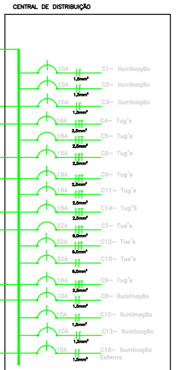
DIAGRAMA UNIFILAR
